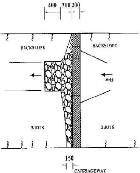
PLAN OF DRAIN WITH SCOUR CHECK
